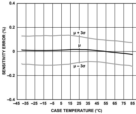
Figure 8. Gyroscope Sensitivity Error, -40°C to +85°C, 1°C/min
