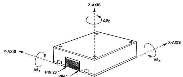
Figure 39. Delta Angle Axis and Polarity Assignments
