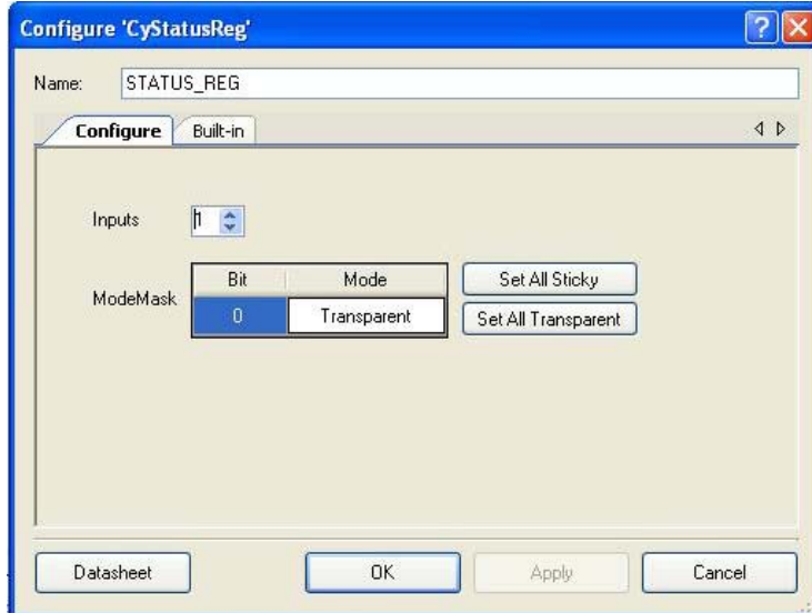
Figure 5-13. STATUS_REG Configuration: Configure Tab
