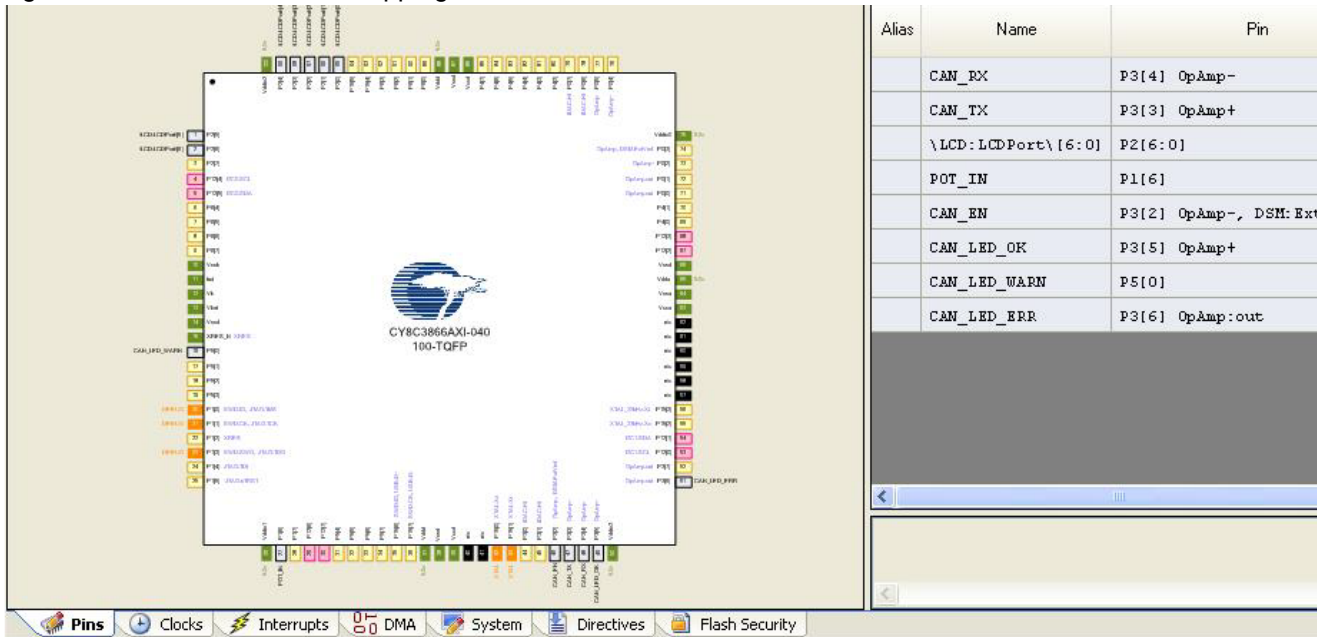
Figure 5-31. Pin Connection Mapping for Port A of CY8CKIT-001 DVK
