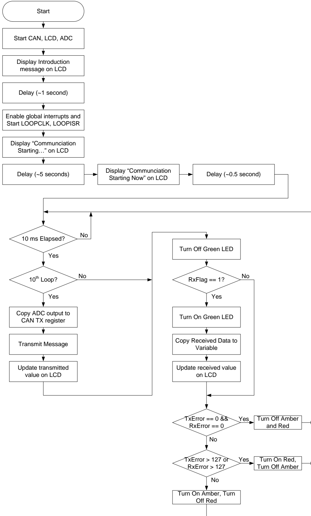
Figure 5-1. Firmware Flowchart
