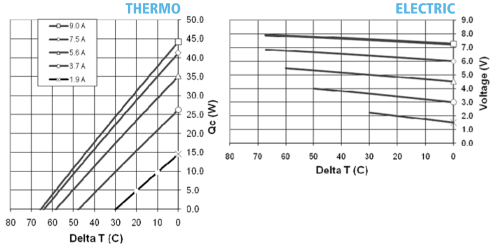
Performance Curves at T_h = 25^\circ\text{C}
