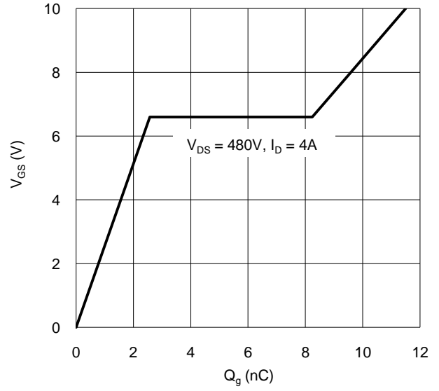
Figure 10. Gate Charge
