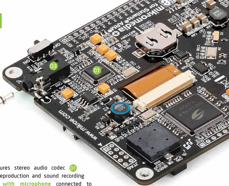
Figure 8-1: On-board VS1053 MP3 codec
