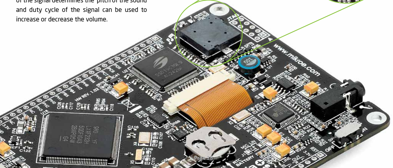
Figure 14-1: Buzzer module
