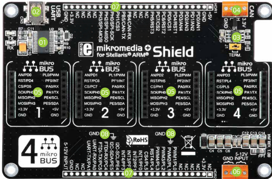
Figure 17-1: mikromedia+ shield
