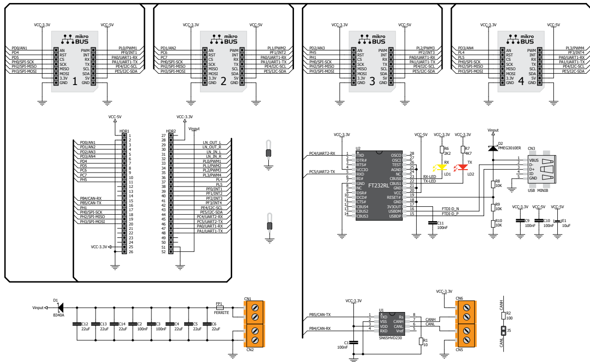
Figure 17-2: mikromedia+ shield schematic
