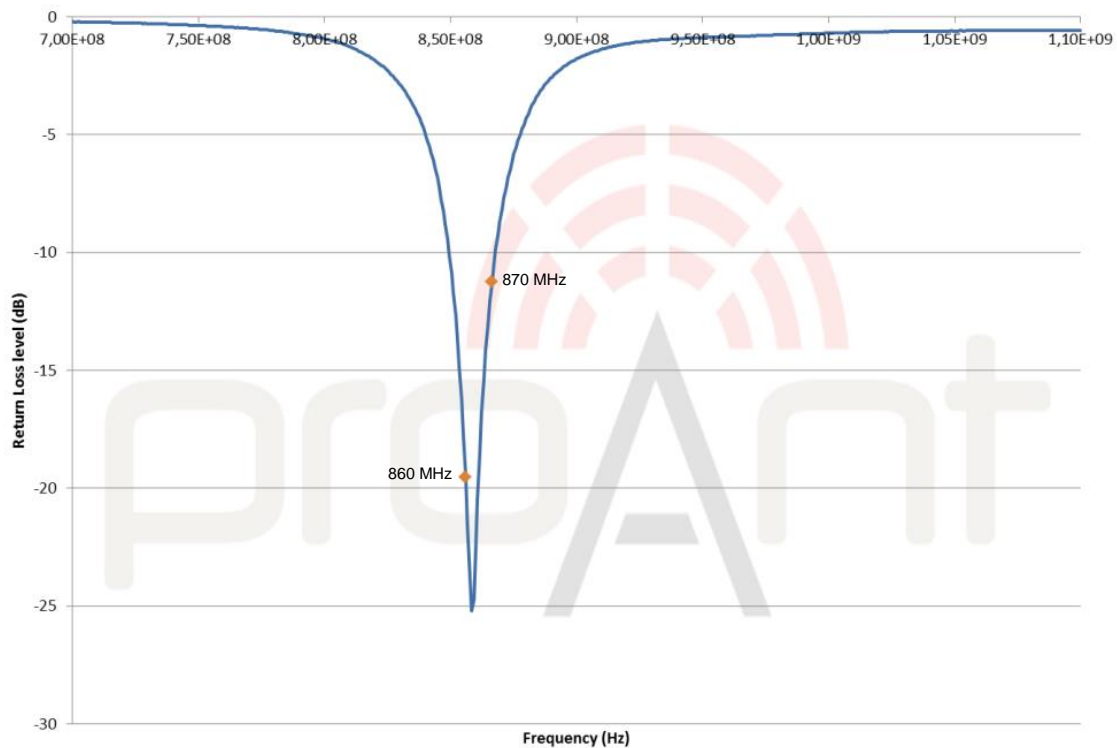
Return Loss
