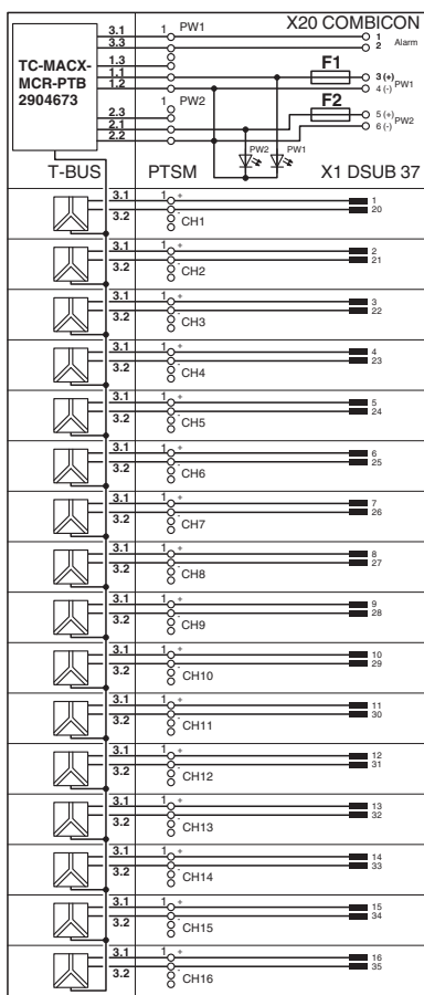
Circuit diagram
